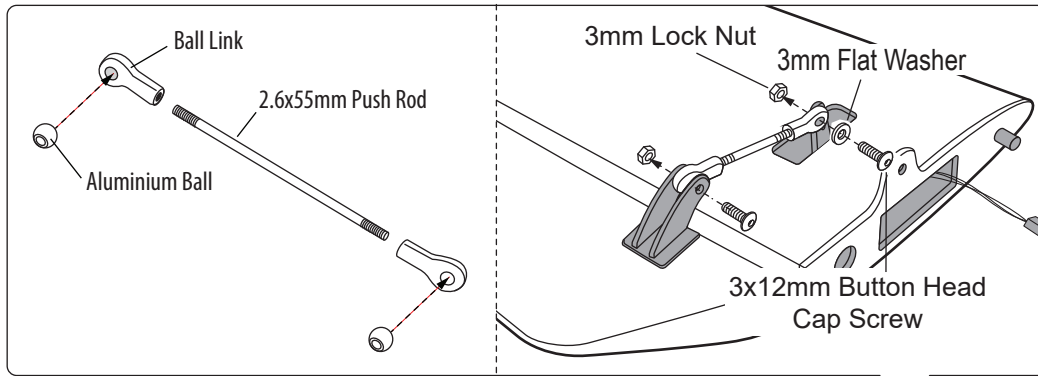
Bottom View
