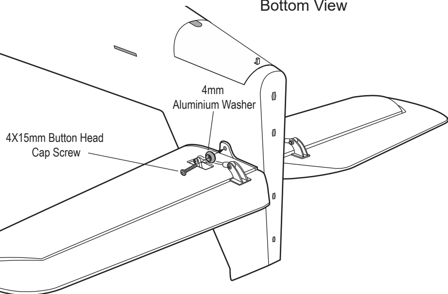
Bottom View
